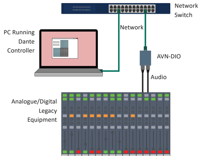
Fig 1-1: Setup
