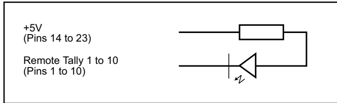
Fig 2-10: Connection Example
