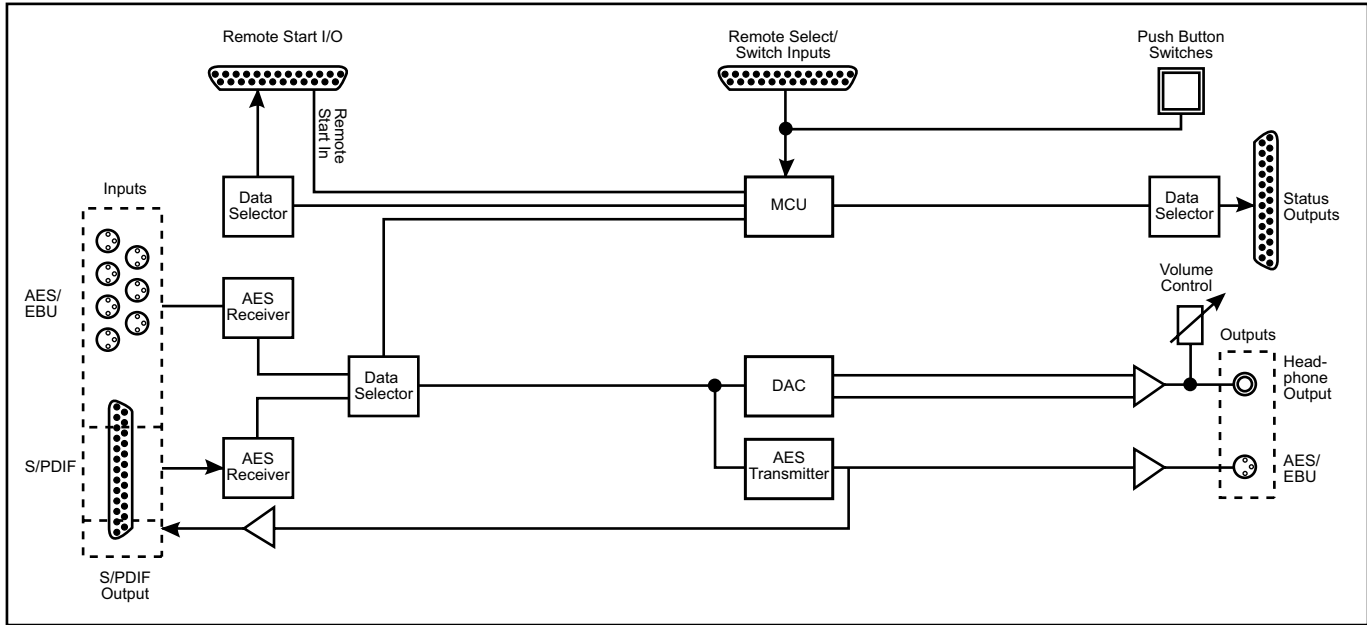
Fig 2-2: RB-DSS10 System Block Diagram
