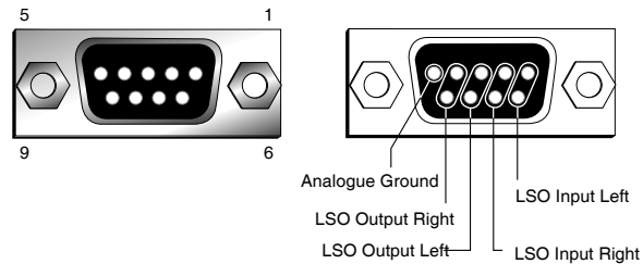
Fig 6-12: RB-OA3 LSO Expansion Connector Details
