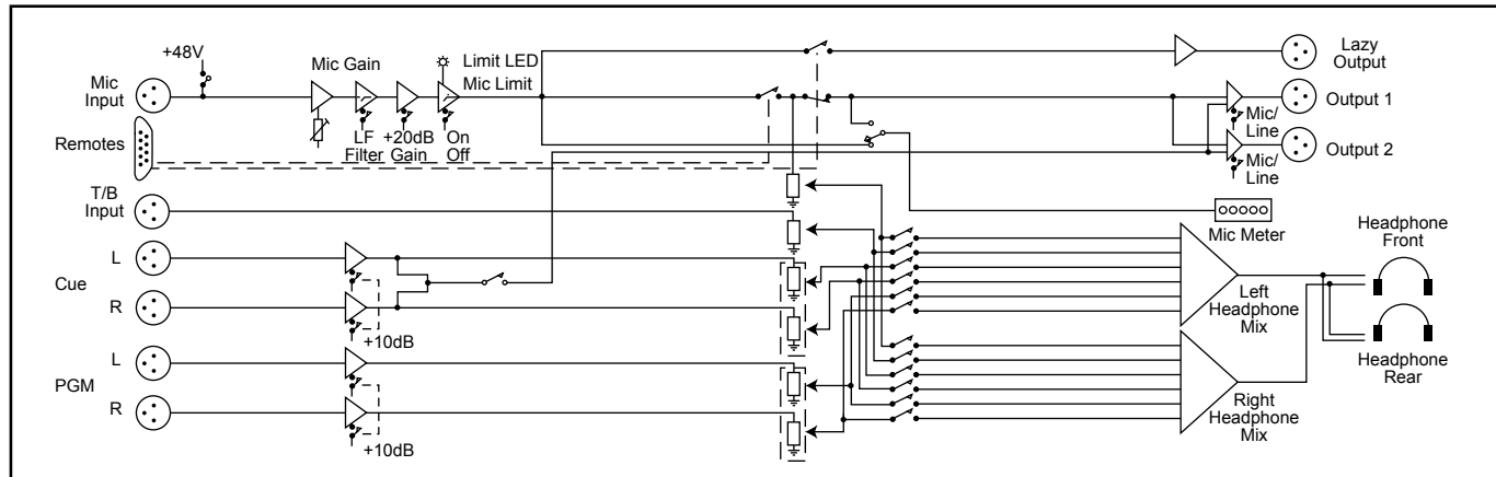
Fig 10-2: RB-MTV1 Block Diagram
