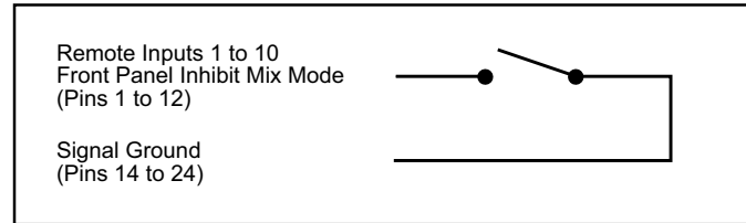
Fig 1-9: Connection Example
