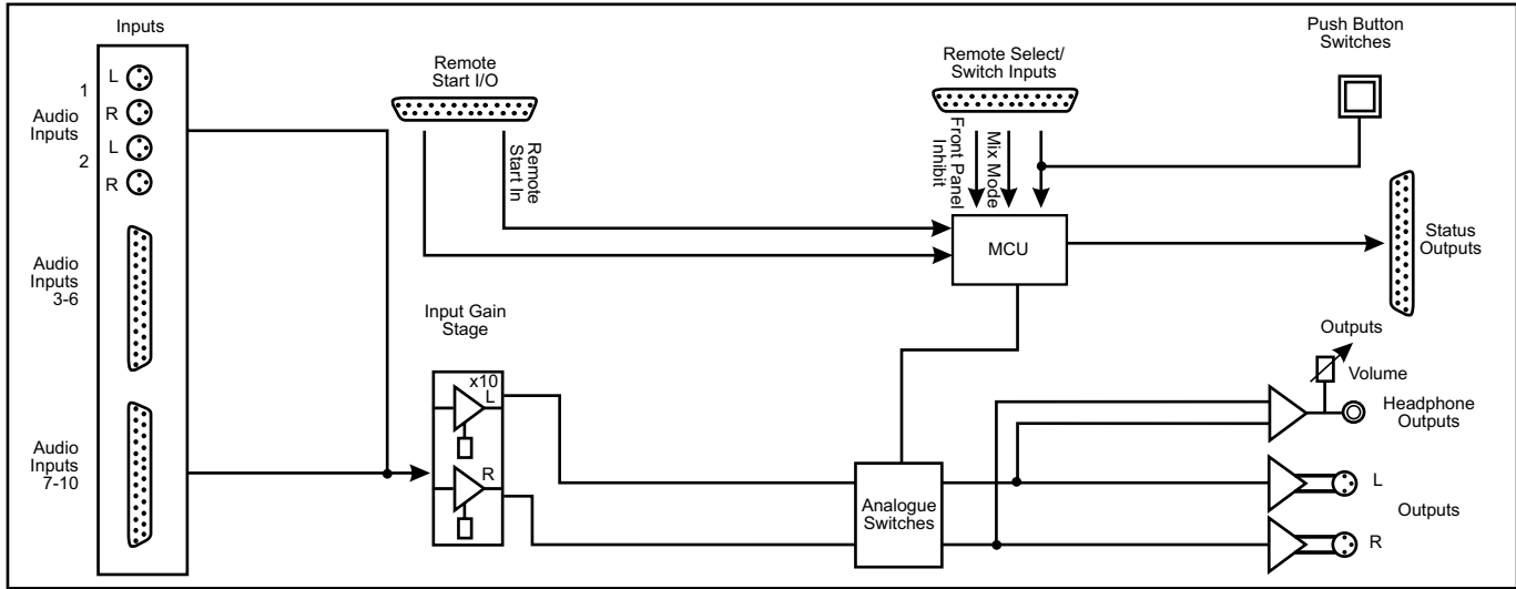
Fig 1-2: RB-SS10 System Block Diagram
