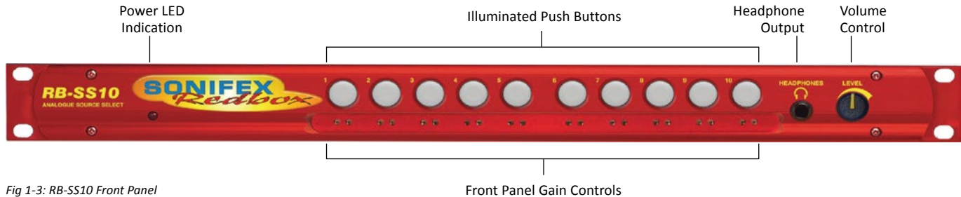
Fig 1-3: RB-SS10 Front Panel
