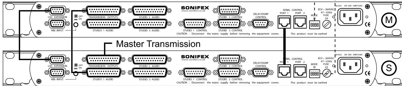
Fig 6-6: RB-OA3 Studio Expansion Diagram
