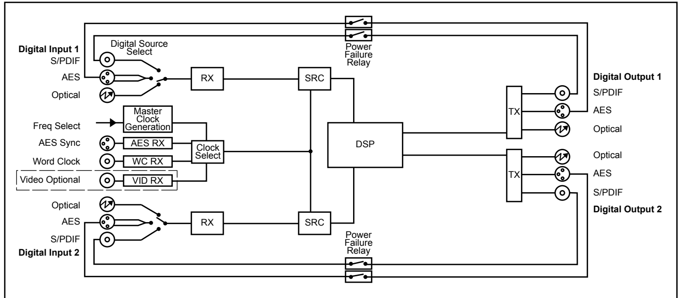
Fig 4-2: RB-DMX4 System Block Diagram
