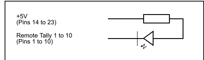
Fig 1-11: Connection Example
