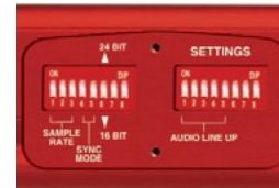
Fig 12-7: DIPSwitch Settings
