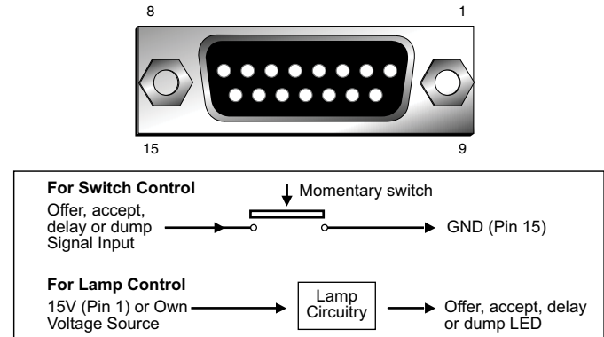
Fig 6-20: RB-OA3 Switch & Lamp Control Details
