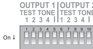
Fig 6-6: RB-DA4x5 Routing Selection Switch
