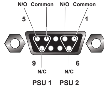
Fig 9-4: RB-DDA6A-2P Alarm Connector Diagram
