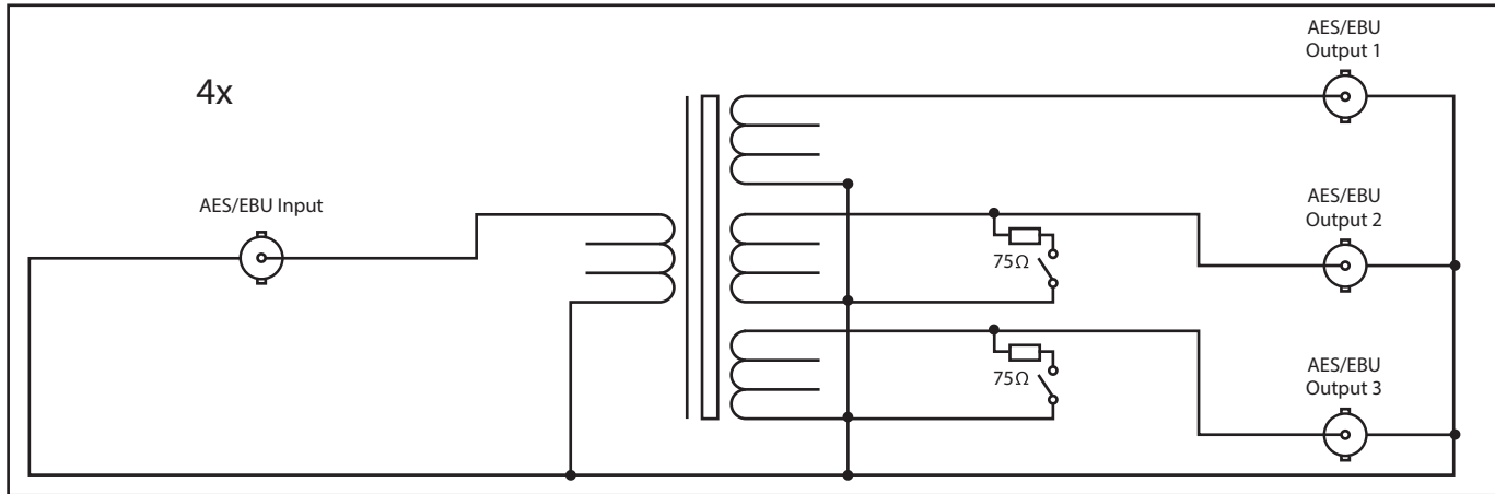
Fig 15-2: RB-AES4B3 System Block Diagram
