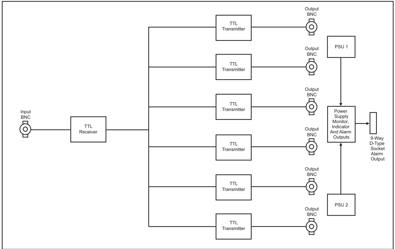
Fig 13-2: RB-DDA6W-2P System Block Diagram
