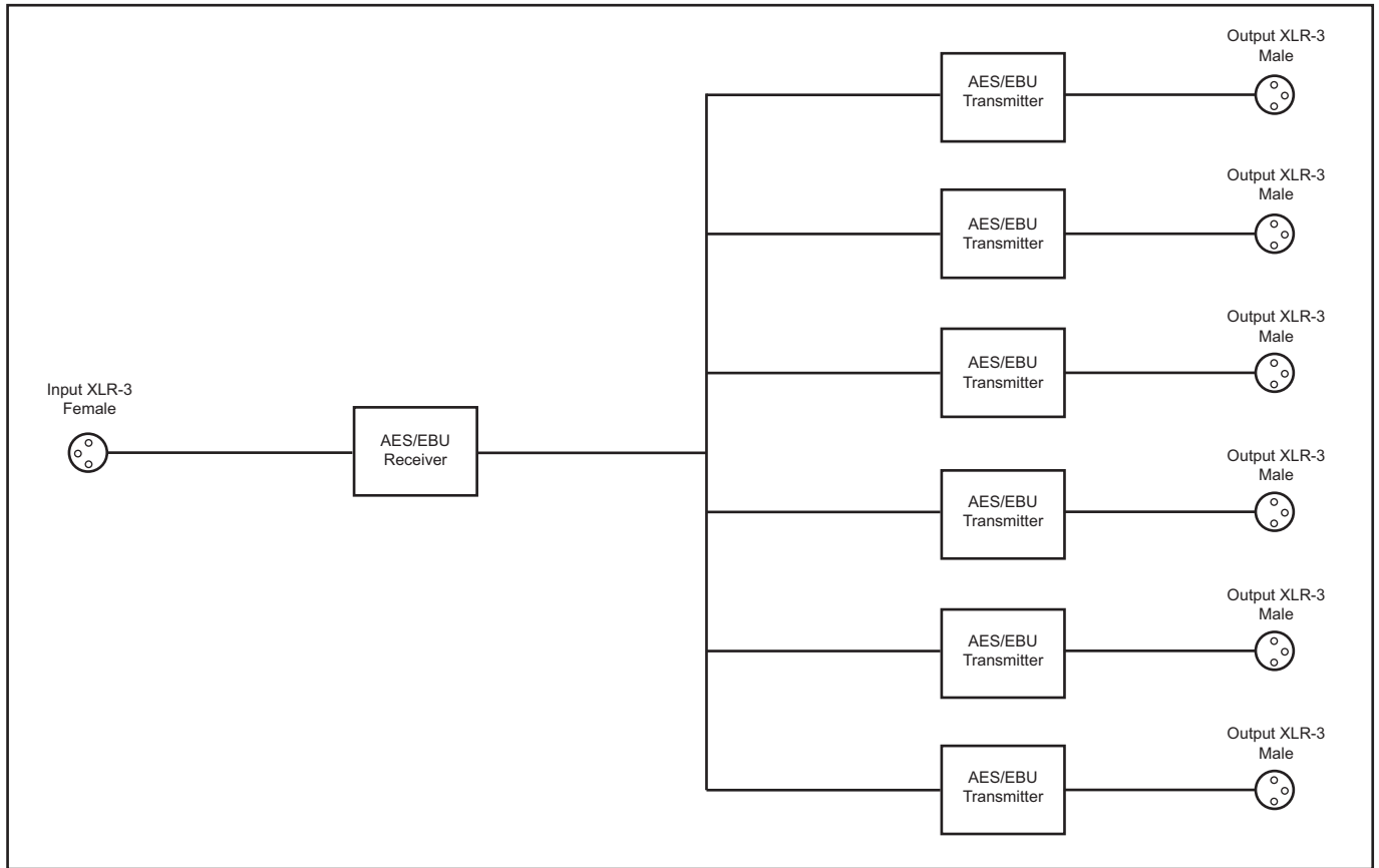
Fig 8-3: RB-DDA6A System Block Diagram
