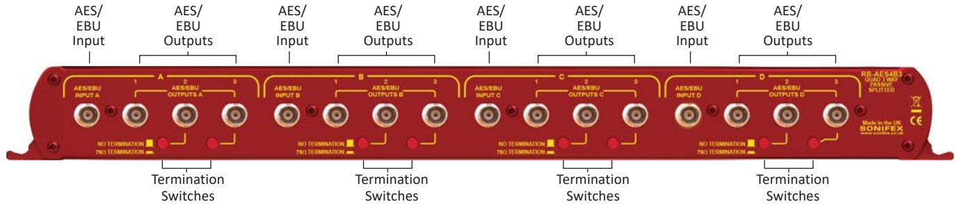
Fig 15-3: RB-AES4B3 Front Rear Panel
