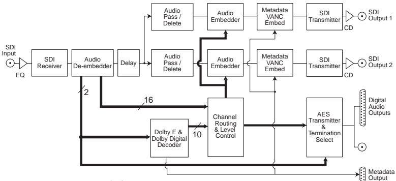
Fig 1-3: RB-VHDDD8 System Block Diagram.
