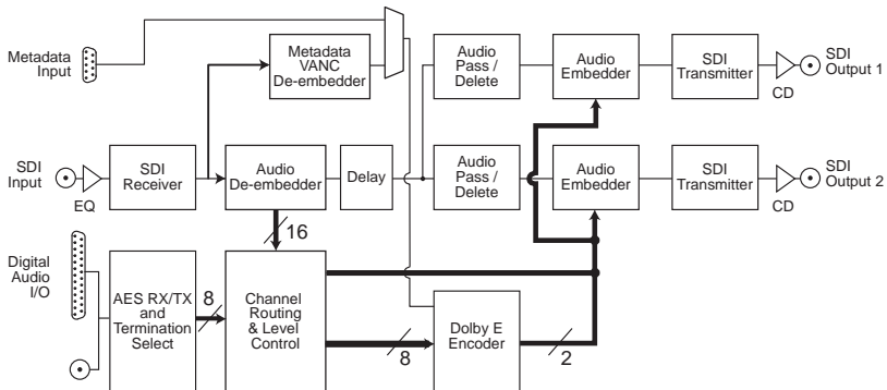
Fig 1-4: RB-VHEDD8 System Block Diagram.
