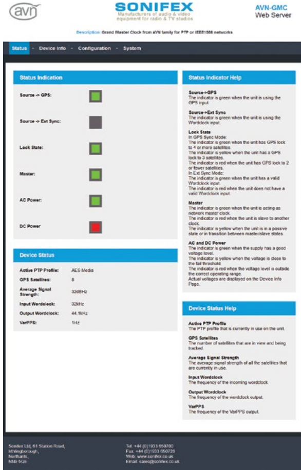
Fig 2-1: Standard Webpage Layout
