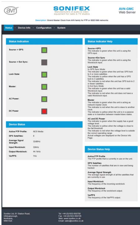
Fig 2-1: Standard Webpage Layout
